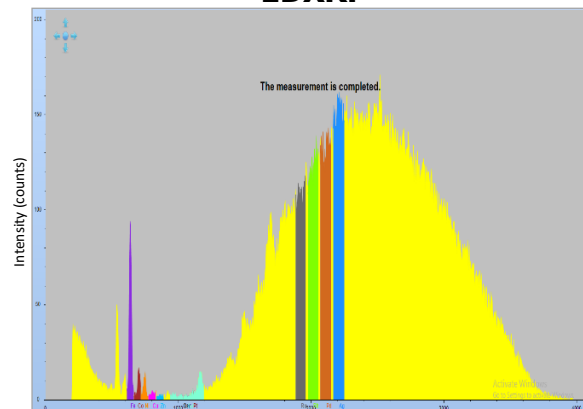
EDXRF
