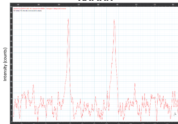
RAMAN
